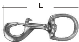
SWIVEL EYE BOLT SNAP casted AISI 316 ITEM NO. Size L mm Weight/g 005005 5/8" (16mm) 90 42 005006 3/4" (19mm) 93 56
